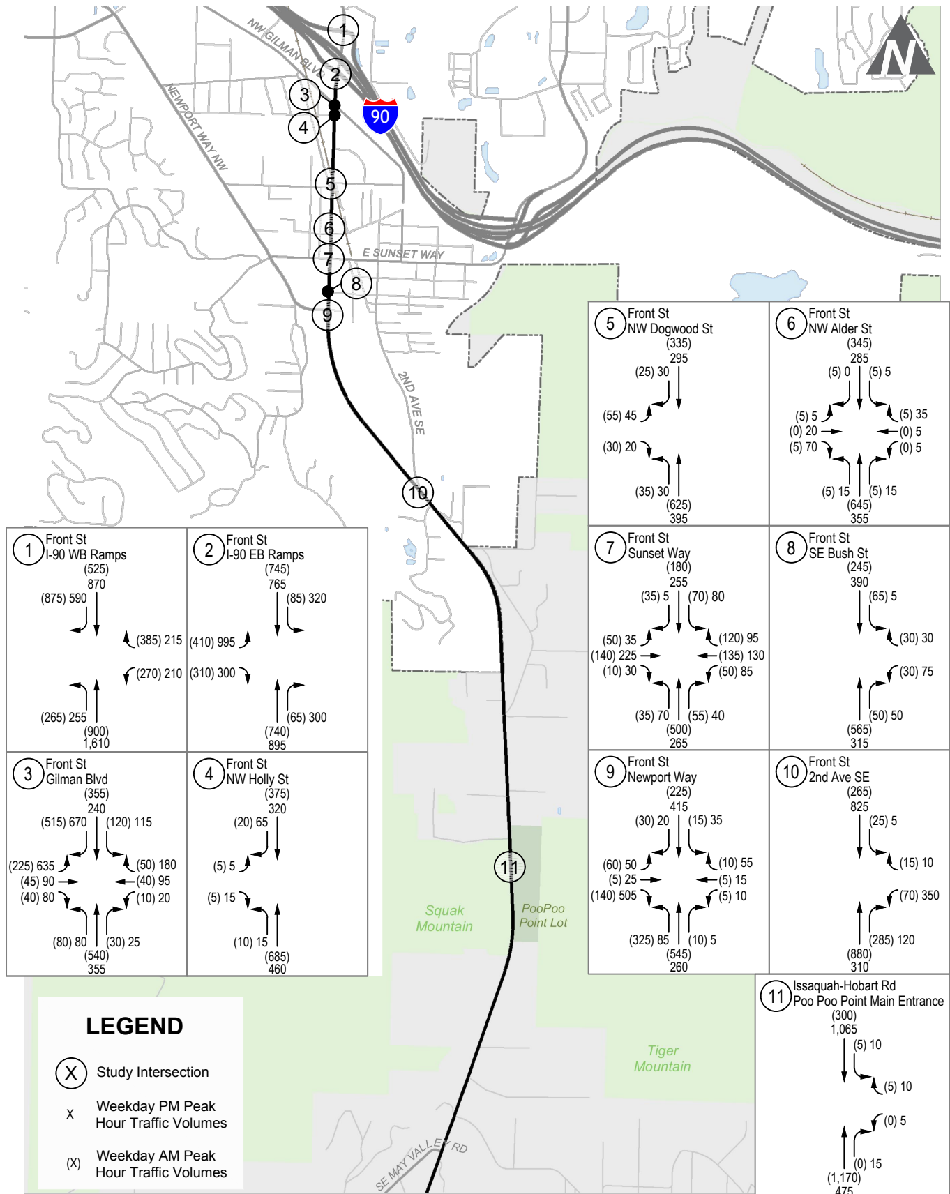
Weekday (2017) AM & PM Peak Hour Traffic Volumes - North
